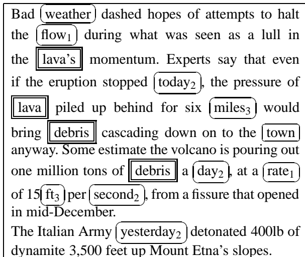
Figure 1: Excerpt of document from our test set with discourse annotations. Centers are in double boxes; terms occurring in lexical chains are in oval boxes. Words with the same subscript are members of the same chain (e.g., today , day , second , yesterday )
