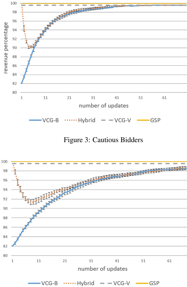
Figure 4: Cautious Bidders, Lax Updates
