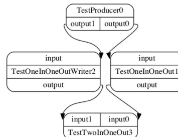
Figure 8: Monitoring service – Detailed job information
