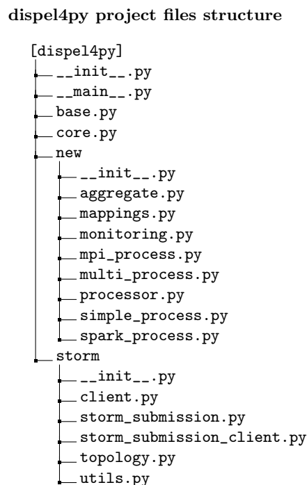
Figure 1: dispel4py project files structure
