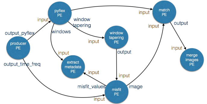
Figure 5: Misfit calculation dispel4py workflow.
