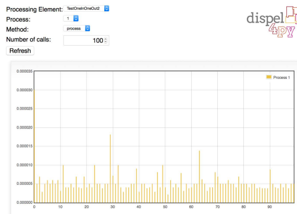
Figure 8: Monitoring service – Detailed job information
