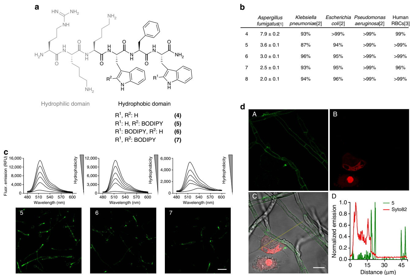
Figure 2 | Fluorogenic peptides for live cell imaging of A.fumigatus in co-culture with human lung epithelial cells. (a) Chemical structures of non-labelled and fluorogenic linear peptides (4–7), highlighting the two conserved hydrophilic (grey) and hydrophobic (black) domains of Peptide Antifungal 26 (PAF26). (b) Activity of antimicrobial peptides in A. fumigatus , several bacterial strains and in human RBCs.[1] IC 50 (μM) values represented as means ± s.e.m. from n = 3 , [2] cell viability upon 16 h incubation with 4–8 at their respective IC 50 concentrations ( n = 3 ), [3] cell viability upon 1 h incubation with 4–8 at their respective IC 50 concentrations ( n = 3 ). (c) Fluorogenic behaviour of 5–7 (10 μM) in phosphatidylcholine (PC):cholesterol (7:1) liposome suspensions in PBS ranging from 3.75 to 0.004 mg ml -1 of PC in two-fold serial dilutions ( \lambda_{exc} : 450 nm), and wash-free live cell images of A. fumigatus at 37 °C using fluorescence confocal microscopy after incubation with peptides 5–7 (5 μM). Scale bar, 20 μm. (d) Peptide 5 (5 μM, green) and Syto82 (2.5 μM, red counterstain for lung epithelial cells) were incubated in co-cultures of A. fumigatus and human lung A549 epithelial cells and imaged under a fluorescence confocal microscope at 37 °C without any washing steps. Fluorescence staining of 5 (A), Syto82 (B), merged (C) and plot profile analysis (D) of peptide 5 (green) and Syto82 (red) from image C. Scale bar, 10 μm.
