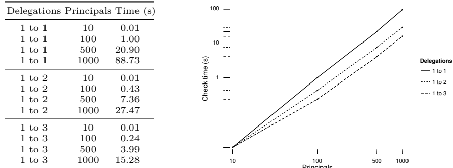
Fig. 5. Benchmarking results on a Nexus 4 Android phone.
