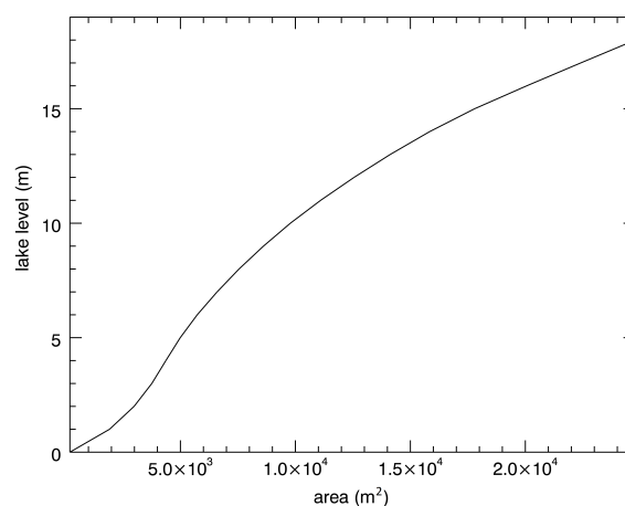
Figure 9. Hypsographic curve of the lake basin derived from the detailed DEM (LB DEM) showing the relation of the lake depth and the lake area.
