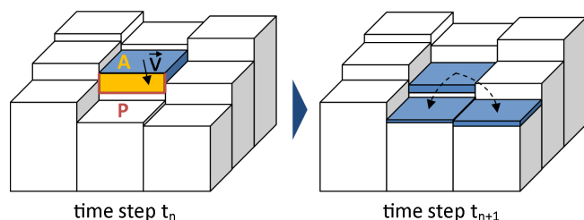
Figure 5. Schematic representation of the concept adopted in the FloodArea HPC model. The block diagrams show the flow between raster cells in time steps t_n and t_{n+1} , indicating flow velocity vector v , cross sectional area A and wetted perimeter P .
