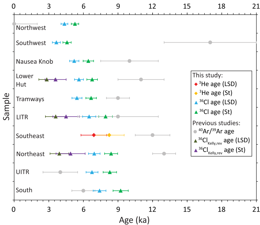
Fig. 7. Exposure ages of the post-caldera lava flows with 1σ total uncertainty versus 40 Ar/ 39 Ar ages from Harpel et al. (2004) and Kelly et al. (2008a) . Only 36 Cl ages are shown for all lava flows except Southeast because the total uncertainty for 36 Cl is significantly smaller than for 3 He. For the Southeast flow, in which a 36 Cl age was not determined, the oldest 3 He age is shown instead. The three 36 Cl ages from Kelly et al. (2008a) , recalculated as described in section 5.6, are also shown with total uncertainty.
