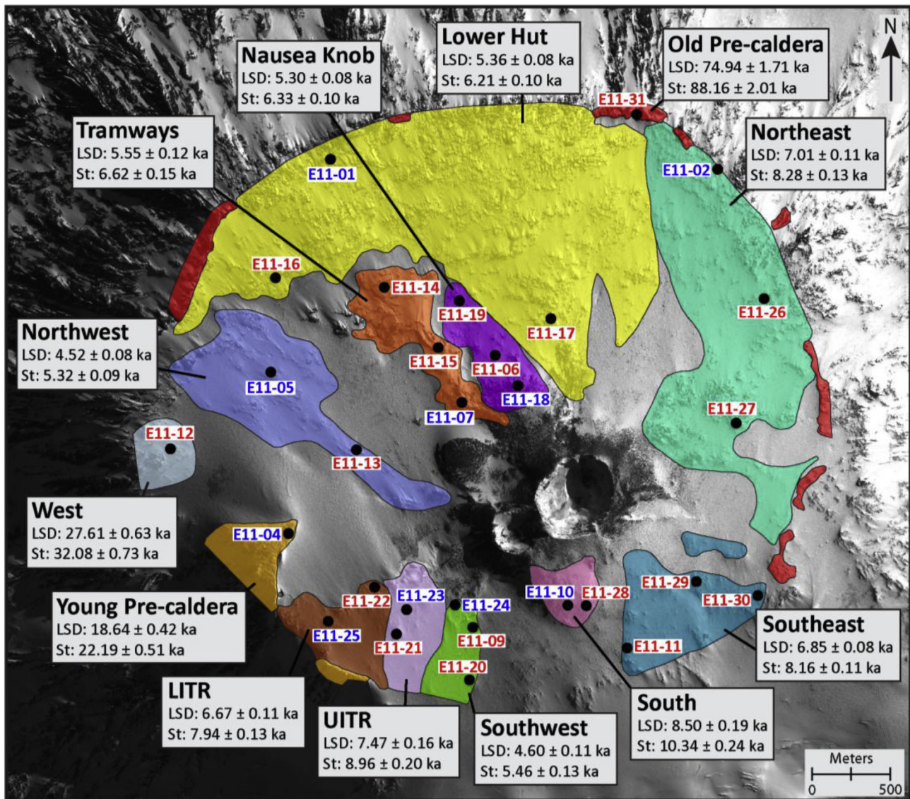
Fig. 2. Map of the Erebus summit caldera lava flows and exposure age sample locations. The lava flows were originally mapped by Caldwell (1989) and Harpel et al. (2004) based on field observations and aerial photographs. All lava flow boundaries are approximate. For each flow, the estimated eruption age and 1\sigma analytical uncertainty, calculated from clinopyroxene ^3\text{He} exposure ages as described in the text (section 5.7), is shown using Lifton et al. (2014) (LSD) and Lal (1991)/Stone (2000) (St) production rate scaling. Blue samples are those dated using both ^3\text{He} and ^{36}\text{Cl} and red samples were dated only using ^3\text{He} . LITR = Lower Ice Tower Ridge, UITR = Upper Ice Tower Ridge. (For interpretation of the references to color in this figure caption, the reader is referred to the web version of this article.)
