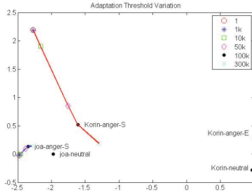
Fig. 4. PCA projection of the different adaptation threshold experiments in the anger cross-lingual extrapolation between joa (Spanish speaker) and Korin (English speaker). The prefix S stands for Spanish and E for English source data. The black dot is the reference system constant across experiments.
