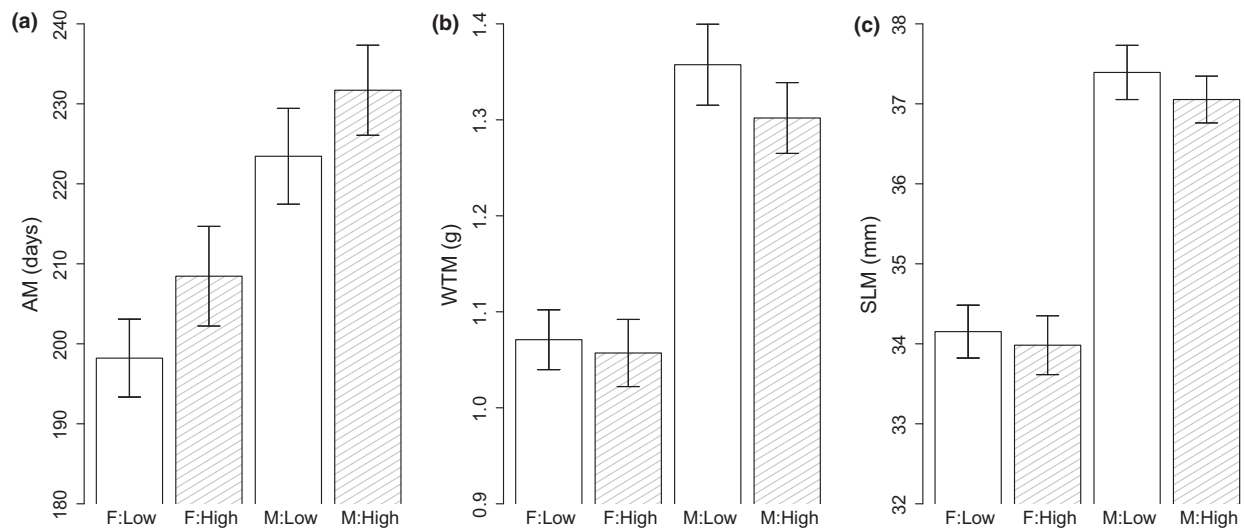
Fig. 2 Mean observed (a) maturation age (AM), (b) weight (WMT) and (c) standard length (MSL) by sex for low- and high-density treatments. White columns denote low (L)-density treatment and shaded columns indicate high (H)-density treatment for male (M) and female (F) values with bars showing mean \pm SE ( n_{FL} = 83 , n_{ML} = 92 , and n_{FH} = 65 , n_{MH} = 103 ).
