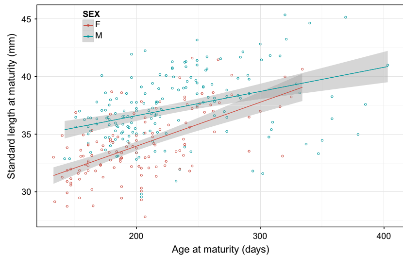
Fig. 1 Observed size (standard length) at maturation as a function of age by sex. Circles denote phenotypic observations ( n_F = 148 , n_M = 195 ) whereas solid lines illustrate predictions from simple linear regressions with shaded areas denoting predicted mean \pm SE.
