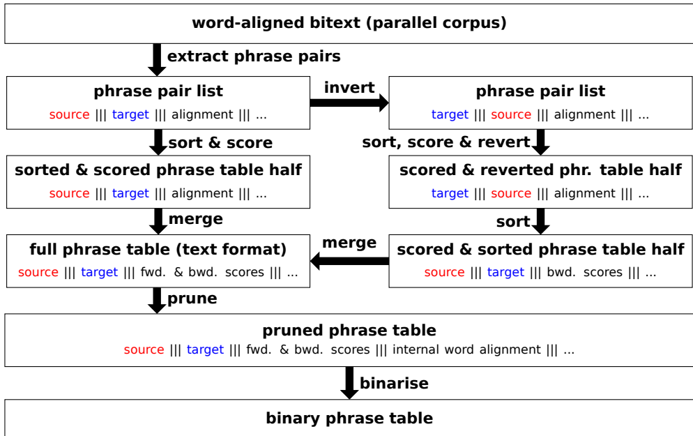
Figure 1. Conventional Phrase Table Construction
