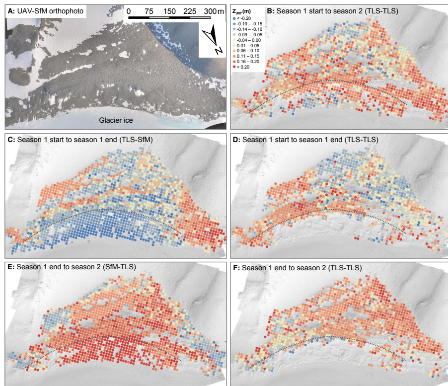
Figure 3. Vertical component of 3-D topographic change ( Z_{diff} ) overlain on a UAV-SfM-derived hill-shaded DEM of the Patriot Hills blue-ice moraine complex. Topographic evolution was quantified using the Multiscale Model to Model Cloud Comparison (M3C2) algorithm in CloudCompare software. (a) UAV-SfM orthophotograph of the study site. Panels (b) to (f) cover specific differencing epochs using a combination of TLS and SfM data (see panel headings). Dashed line in (b) to (f) indicates locations of primary moraine ridge crest.
