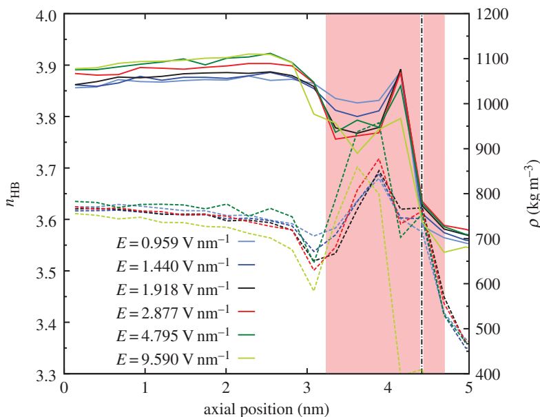
Figure 14. Axial density profiles (continuous lines) and average number of hydrogen bonds per water molecule (dashed lines) for various values of applied field strength \mathbf{E} . The pink shaded area shows where the electric field is applied, while the vertical dotted-dashed black line indicates the entrance of the CNT. (Online version in colour.)
