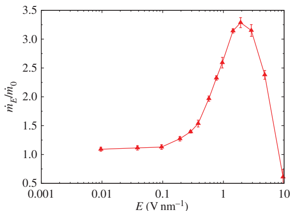
Figure 13. Mass flow rate \dot{m}_E/\dot{m}_0 measured for various electric field magnitudes \mathbf{E} in Case C simulations. Measurements along the nanotube are made in a cylinder of radius 0.7 nm, centred on the nanotube axis, in the streamwise direction. Error bars show 2 s.d. of the samples (95% CI). (Online version in colour.)
