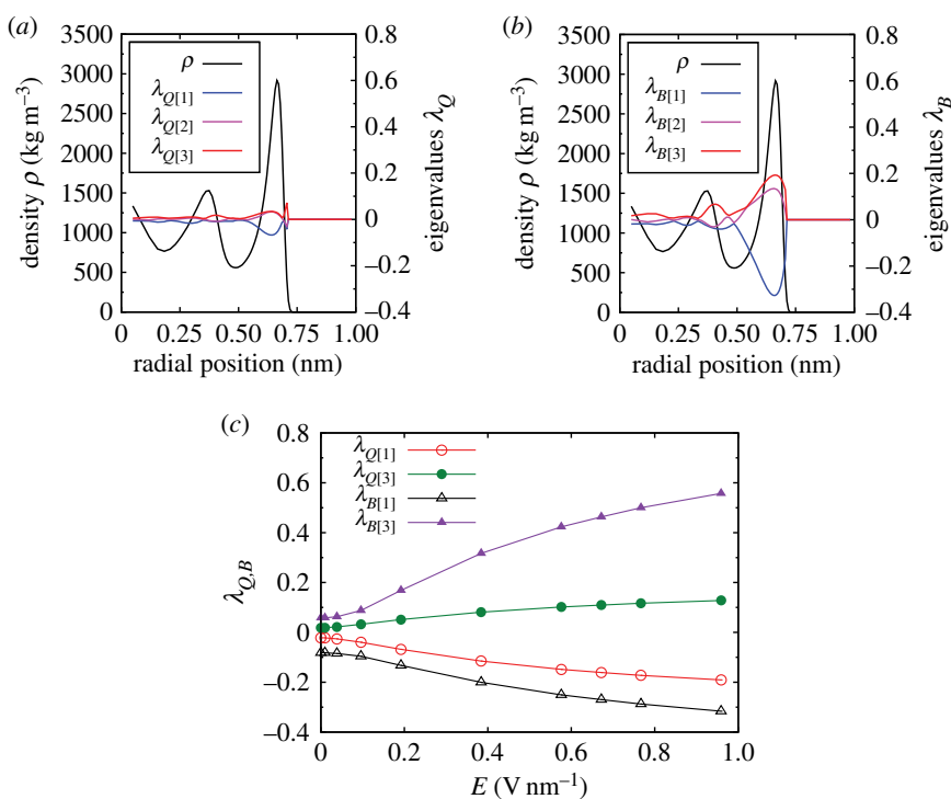
Figure 3. (a) Water density profile and eigenvalues \lambda_Q of the order tensor \mathbf{Q} , and (b) water density profile and eigenvalues \lambda_B of the order tensor \mathbf{B} , as a function of radial distance from the centre of the CNT axis, averaged over the length of the CNT for the zero-field situation. (c) Maximum and minimum eigenvalues \lambda_{Q,B} of the order tensors when the electric field is applied over the whole system (Case A). The standard error of the mean (s.e.m.) with 95% confidence interval (CI) is smaller than the symbol. (Online version in colour.)
