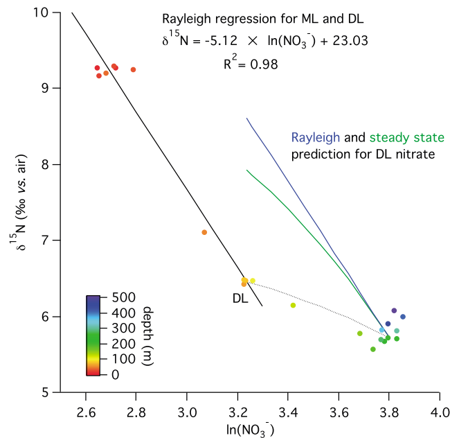
Figure 5. The summer mixed layer (ML) to DL nitrate concentration and \delta^{15}\text{N} from station K1 (same data set from Figure 3a), when interpreted with the Rayleigh model (black solid line), suggest that the isotope effect for nitrate assimilation is \sim 5.1\text{‰} , as given by the slope of the regression. However, the \delta^{15}\text{N} of the DL nitrate is much lower than the Rayleigh model (blue line) or steady state model (green line) predictions under the assumptions (1) that the thermocline nitrate between 200 and 300 m is the source for winter mixed layer and (2) there is a similar isotope effect of 5.1\text{‰} during winter nitrate assimilation. The Rayleigh model assumes the consumption of a substrate in a closed system with constant isotopic fractionation, and the steady state model assumes that the net nitrate supply to the upper ocean (including the surface mixed layer and the underlying DL) is balanced by sinking organic N. The lower than predicted nitrate \delta^{15}\text{N} of the DL may be the result of remineralization of low- \delta^{15}\text{N} suspended PN within the DL (see text) [Smart et al., 2015].
