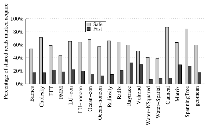
Figure 7. Static percentage of potentially thread-escaping reads that our analysis marks as an acquire.
