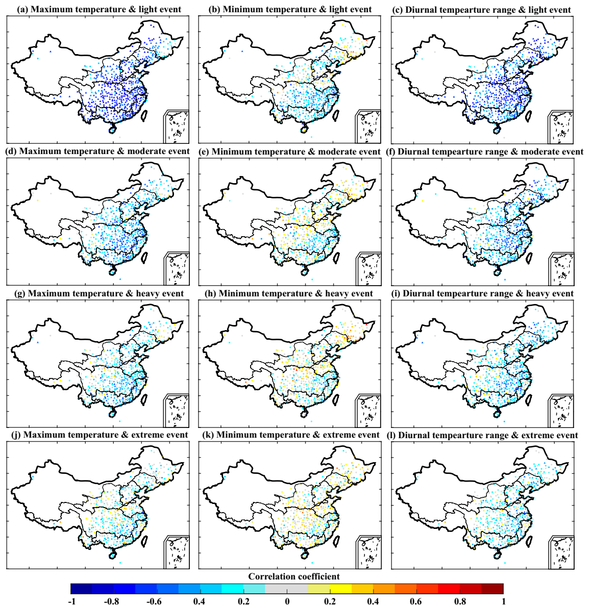
Figure 7. Spatial patterns of the correlations between temperature variations and the frequency of hourly light, moderate, heavy, and extreme precipitation events. The triangles indicate correlation coefficients that were statistically significant at the p < 0.05 level. The maps were created using MATLAB ( http://www.mathworks.com ).
