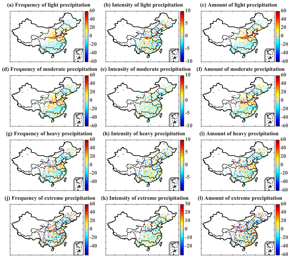
Figure 1. Percentage changes across mainland China in frequency, intensity, and total precipitation amount for hourly light, moderate, heavy, and extreme precipitation events between the periods 1991–2001 and 2002–2012. The maps were created using MATLAB ( http://www.mathworks.com ).
