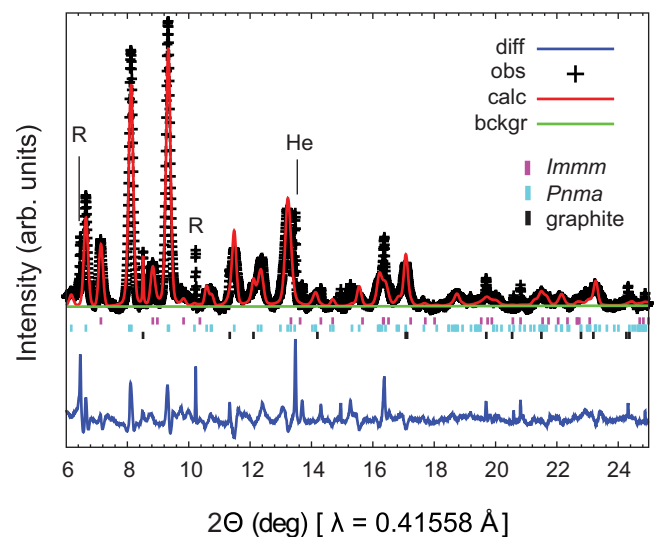
FIG. 4. (Color online) Rietveld refinement of the synchrotron PXRD pattern of Pnma \text{Li}_2\text{C}_2 at 18.7 GPa ( \lambda = 0.41558 \text{ \AA} ). Experimental data points (+), calculated profile (red solid line), and difference curve (blue curve below) are shown. Vertical bars mark the positions of Bragg reflections of graphite (black), Pnma \text{Li}_2\text{C}_2 (light blue), and Immm \text{Li}_2\text{C}_2 (magenta). Sharp extra reflections stem from ruby (R) and the PTM He.
