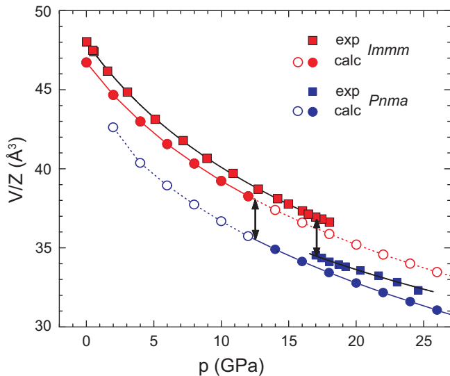
FIG. 5. (Color online) Volume versus pressure data for Immm \text{Li}_2\text{C}_2 (red symbols) and Pnma \text{Li}_2\text{C}_2 (blue symbols). Experimental and computed values are presented as squares and circles, respectively. The transition pressures are marked by arrows.
