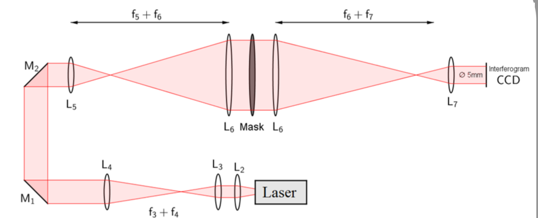
Figure 6 (above). Spatial coherence measurement using NRA mask and achromatic doublet beam expanding lenses.
