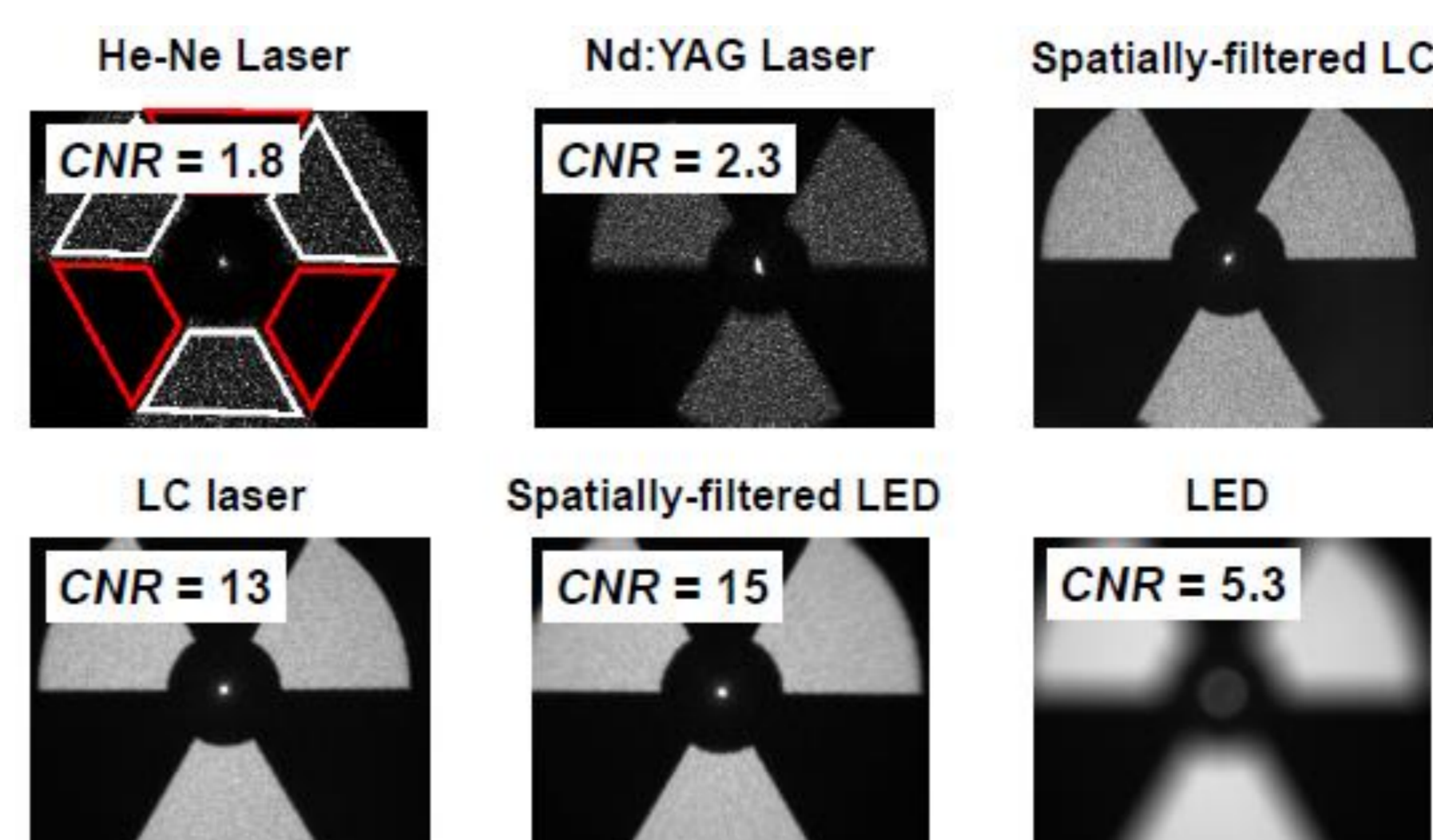
Figure 10. Reconstructed images from a multi-level phase hologram captured in the replay field for the different light sources. The foreground regions used in the above equation are shown in white on the He-Ne image, the background are shown in red.
