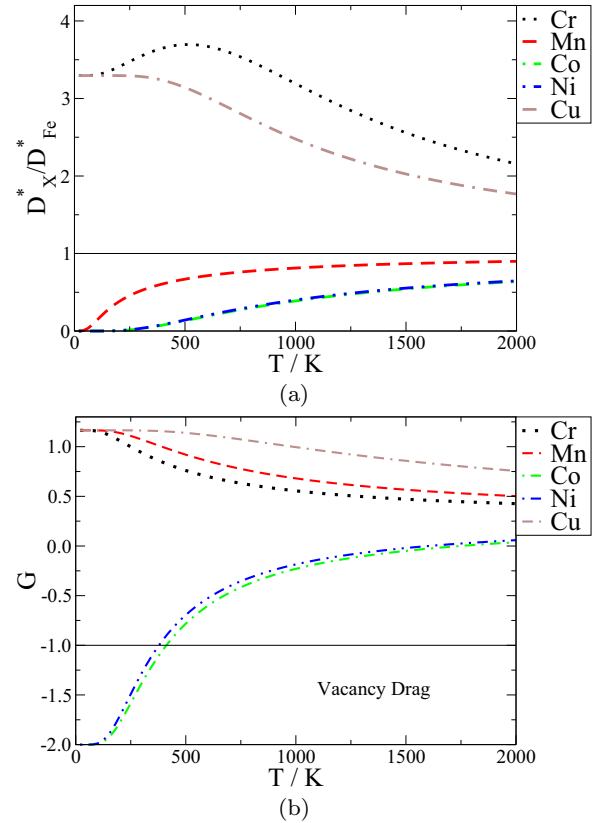
FIG. 10. (Color online) Temperature dependence of (a) the tracer diffusion coefficient ratio, D_X^*/D_{\text{Fe}}^* , and (b) the vacancy wind parameter, G , for the solutes Cr (black, dotted line), Mn (red, dashed line), Co (green, dot-dashed line), Ni (blue, double-dot-dashed line), and Cu (brown, dot-double-dashed line). Data, including errors, are given in Table II. The line in (b) shows the vacancy drag regime ( G < -1 ).
