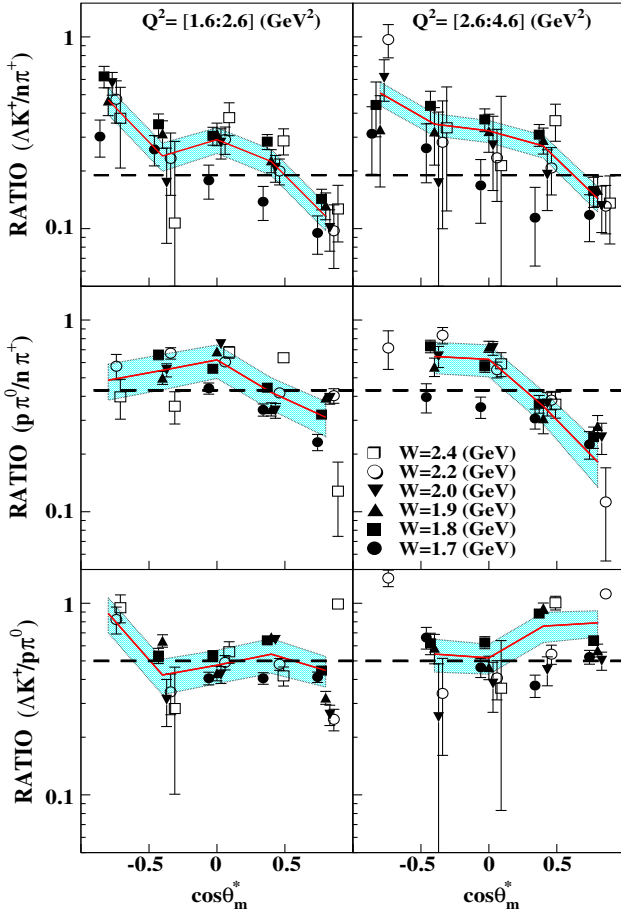
FIG. 1 (color online). Ratio of the three exclusive cross sections, \Delta K^+ to n\pi^+ (top), p\pi^0 to n\pi^+ (middle), and \Delta K^+ to p\pi^0 (bottom), for bins of \langle Q^2 \rangle = 1.9 \text{ GeV}^2 (left) and \langle Q^2 \rangle = 3.2 \text{ GeV}^2 (right), plotted versus \cos\theta_m^* with different bins in W shown as different symbols. The systematic uncertainty is indicated by the shaded band, centered on the solid (red) line which connects the statistically weighted average for each bin. The flat dashed line represents the overall statistical average for each ratio. The data points are plotted slightly offset for clarity.
