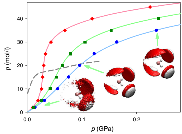
FIG. 3 (color online). Density of water along the T = 673 , 773 , and 873 K isotherms (from top to bottom) as obtained in APIMD QDO simulation (symbols) versus experimental data (full lines). All simulated states, apart from the first four in each isotherm, are in the supercritical region [2]. The dashed line indicates the crossover densities. 3D plots (insets) showing first oxygen (red) and hydrogen (white) coordination shells, illustrate remarkable persistence of tetrahedral structure at T = 673 K.
