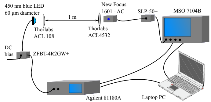
Fig. 9. Experimental set-up.
