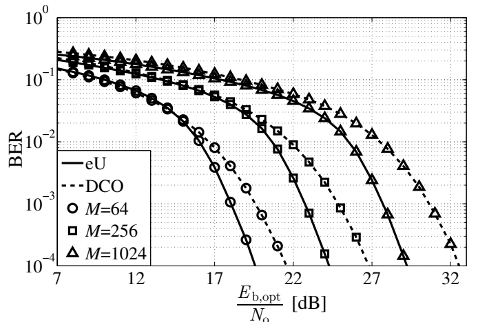
Fig. 8. eU-OFDM performance vs. DCO-OFDM performance for different M -QAM constellation sizes as a function of the optical SNR. Optimum biasing levels for 64-QAM, 256-QAM, and 1024-QAM DCO-OFDM are estimated at respectively 9.5 dB, 11 dB, and 13 dB, as described in (4).
