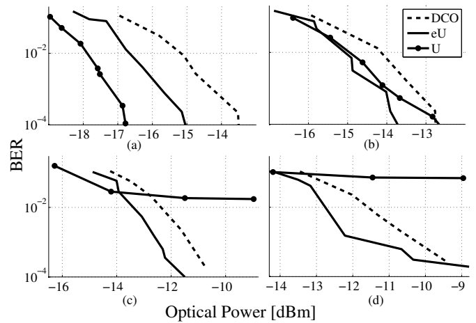
Fig. 13. Performance comparison between eU-OFDM, U-OFDM, and DCO-OFDM for different M -QAM constellation sizes as a function of the optical power measured at the receiver: (a) BPSK (20 Mb/s); (b) 4-QAM (40 Mb/s); (c) 8-QAM (60 Mb/s); (d) 16-QAM (80 Mb/s). All results have been optimized empirically using exhaustive search experiments.
