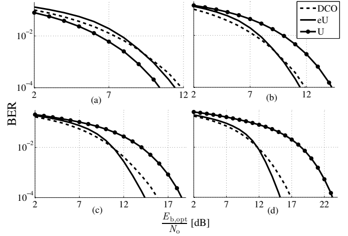
Fig. 7. Performance comparison between eU-OFDM, U-OFDM, and DCO-OFDM for different M -QAM constellation sizes as a function of the optical SNR: (a) BPSK; (b) 4-QAM; (c) 8-QAM; (d) 16-QAM. Optimum biasing levels for BPSK, 4-QAM, 8-QAM, and 16-QAM DCO-OFDM are estimated through Monte Carlo simulations at respectively 6 dB, 6 dB, 7 dB, and 7.5 dB, as described in (4).
