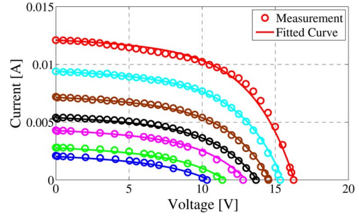
Fig. 6. Measured and fitted I-V curves of the solar panel under various light irradiance. From top to bottom, the light irradiance levels are: 1.184 \times 10^{-2} W/cm 2 , 8.291 \times 10^{-3} W/cm 2 , 5.922 \times 10^{-3} W/cm 2 , 4.401 \times 10^{-3} W/cm 2 , 3.383 \times 10^{-3} W/cm 2 , 2.186 \times 10^{-3} W/cm 2 , 1.561 \times 10^{-3} W/cm 2 .
