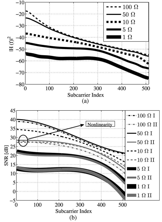
Fig. 13. Experimental SNR estimation for OFDM using Estimator I and Estimator II. (a) Estimated channel. (b) Estimated SNR.
