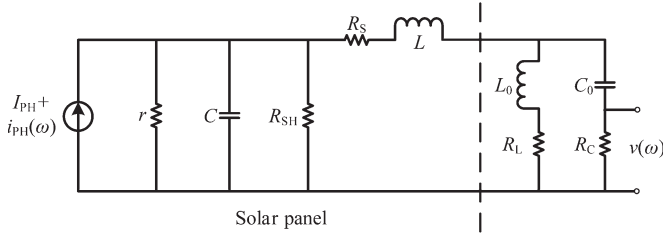
Fig. 3. Solar panel configuration for simultaneous energy harvesting and communication.
