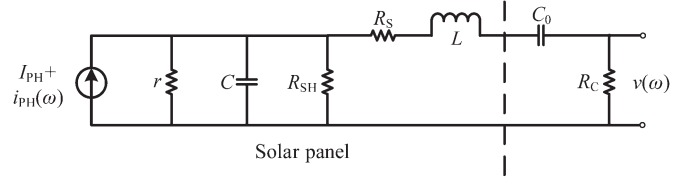
Fig. 2. Solar panel model for communication.
