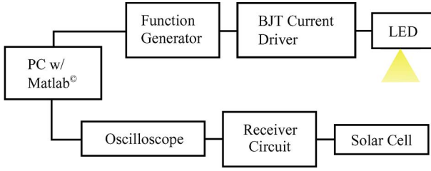
Fig. 10. Experimental setup.
