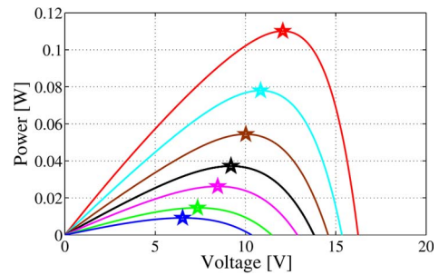
Fig. 7. Estimated P-V curves of the solar panel under various light irradiance levels. Star: maximum power point. From top to bottom, the light irradiance levels are: 1.184 \times 10^{-2} W/cm 2 , 8.291 \times 10^{-3} W/cm 2 , 5.922 \times 10^{-3} W/cm 2 , 4.401 \times 10^{-3} W/cm 2 , 3.383 \times 10^{-3} W/cm 2 , 2.186 \times 10^{-3} W/cm 2 , 1.561 \times 10^{-3} W/cm 2 .
