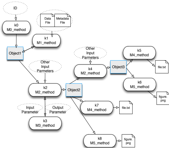
Fig. 8: Algebra of operations.
