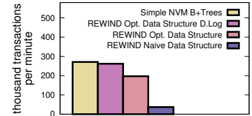
Figure 11: TPC-C throughput.
