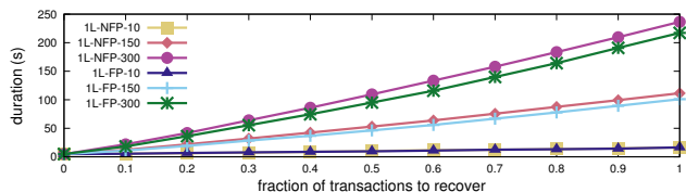
Figure 5: Logging and recovery cost as a function of the fraction of recovered transactions.
