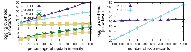
Figure 3: Logging overhead as a function of update intensity (left) and number of skip records (right).
