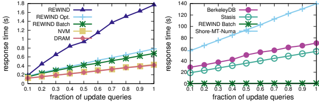
Figure 7: B + -tree logging performance for REWIND vs. no recoverability (left); REWIND vs. Stasis, BerkeleyDB and Shore-MT (right).
