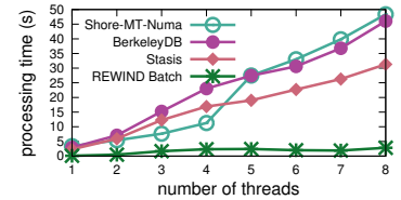
Figure 9: Multithreaded B + -tree logging performance.
