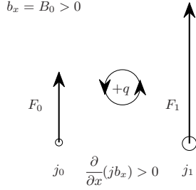
FIGURE 2. A pictorial representation of how the vorticity is generated by the Lorentz term \mathbf{j} \times \mathbf{B} = \nabla \cdot (j\mathbf{B}) in two-dimensional incompressible MHD; see text for details.
