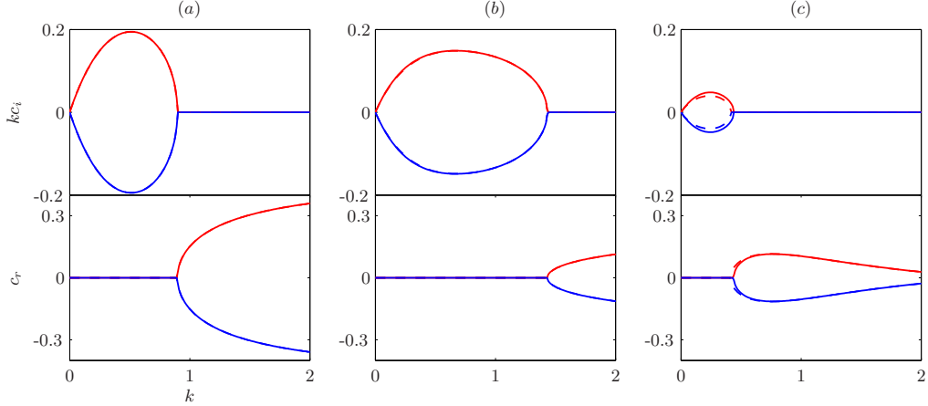
FIGURE 9. Line plots of the growth rate kc_i (top row) and the phase speed c_r (bottom row) associated with the growing and decaying solutions of the full solution (4.14), denoted by solid lines, and the \chi = 0 solutions (4.17), denoted by dashed lines. These are evaluated at fixed M , with (a) M = 0.5 , (b) M = 0.75 , and (c) M = 0.9 . The \chi = 0 solution is, for the most part, indistinguishable from the analytical solution.
