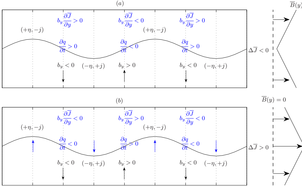
FIGURE 4. Pictorial representation for wave dynamics associated with b_y(\partial\bar{J}/\partial y) , the third term on the right hand side of (2.5a), with (a) \bar{B}\Delta\bar{J} < 0 and (b) \bar{B}\Delta\bar{J} > 0 ; without loss of generality, \bar{B} > 0 . The initial conditions are given in black, and the resulting tendencies arising from the choice of initial conditions are given in blue. See text for more details.
