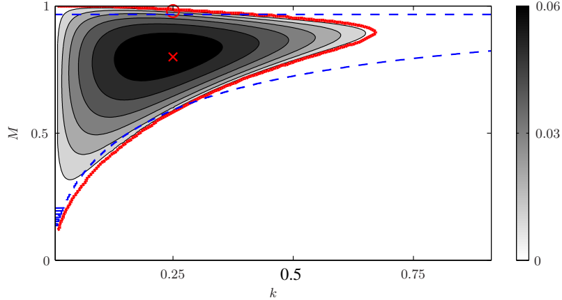
FIGURE 10. Growth rates (kc_i)_{\text{full}} of the full numerical solution associated with the basic state (5.1). Here, c_r = 0 for all unstable modes. The red cross and circle correspond to the parameter location associated with the eigenfunction displayed in figure 11a,b respectively. The thick red line is the stability boundary, and the blue dashed curve is the resonance condition given in (5.3); numerical noise is present at small k partly due to the form of the phase speed c_A .
