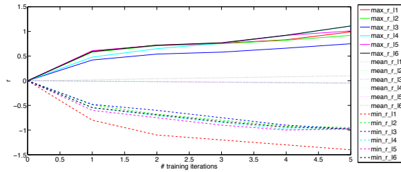
Fig. 4. Maximum, mean, and minimum values of r for one of the speakers in test2010 ; r = 0 corresponds to a gain of 1.
