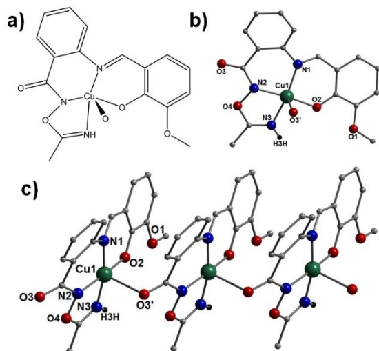
Figure 10 (a) ChemDraw representation and crystal structure (b) of one [Cu(II)(L_4)] unit in 6 including the next bridging oxygen ( O3' ) atom. (c) Representation of the repeating 1D structure in 6 (comprising three [Cu(II)(L_4)] units). The majority of hydrogen atoms and all H_2O solvents of crystallisation were omitted for clarity.
