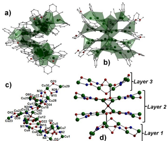
Figure 8 a) and b) Two perspectives of the cluster in 5 as viewed in polyhedral mode. All hydrogen atoms have been omitted for clarity. (c and d) Two perspectives of the inorganic core in 5 . Image d shows the three distinct near planar layers forming the core. The long Cu-O contacts linking the layers are given as thick black lines.
