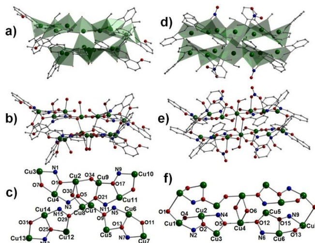
Figure 4 Polyhedral and standard representations of the crystals in 2 (a and b respectively) and 4 (d and e respectively). All hydrogen atoms have been omitted for clarity. The \text{NO}_3^- counter anions in 2 were also omitted for clarity. Figures c and f represent the inorganic cores in 2 and 4 respectively.
