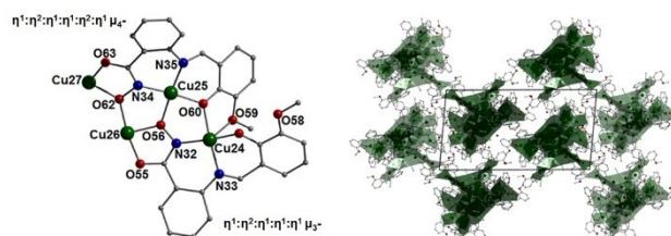
Figure 9 (left) The two distinct bonding modes exhibited by the \text{L}_1^{3-} ligands in [\text{Cu}_{30}] ( 5 ). (right) Packing of the crystals in 5 as viewed along the a cell direction. All hydrogen atoms and perchlorate counter anions have been omitted for clarity.
