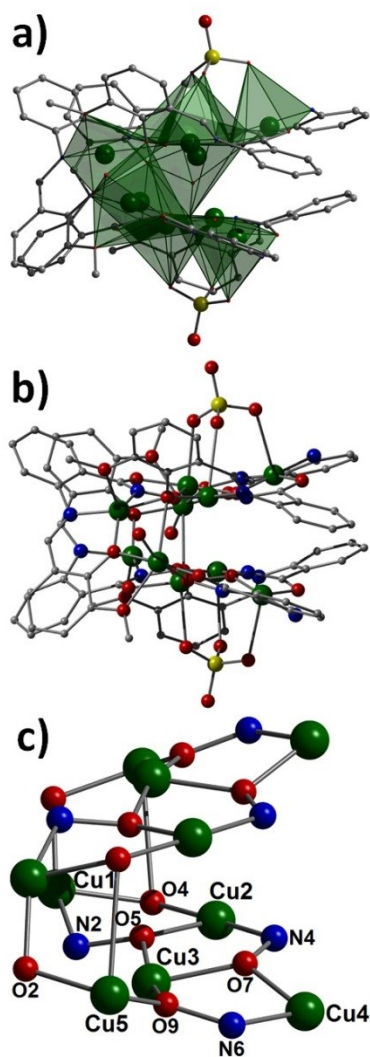
Figure 1 Polyhedral (a) and standard (b) representation of the crystal structure in 1. All hydrogen atoms have been omitted for clarity. (c) The inorganic core in 1. Colour code (used throughout this work): Green (Cu), Red (O), Blue (N), Grey (C) and Yellow (Cl).
