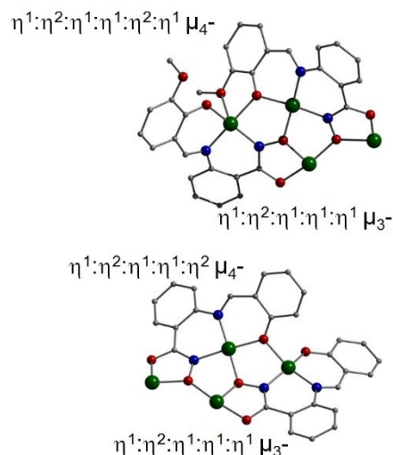
Figure 6 The two different bonding modes exhibited by the L 1 3- ligands in 2 (top) and L 3 3- ligands in 4 (bottom). All hydrogen atoms have been omitted for clarity.
