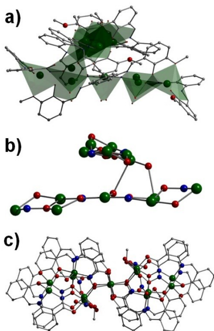
Figure 5 The criss-cross orientation of the {Cu 7 } planes in 2 and 3 (a and b) as opposed to the pseudo superimposable stacking arrangement observed in 4 (c).
