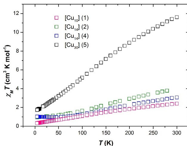
Figure 11 Plots of \chi_M T vs. T for complex 1 , 2 , 4 and 5 .
