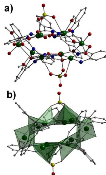
Figure 2 Alternative perspective of 1. All hydrogen atoms have been omitted for clarity.
