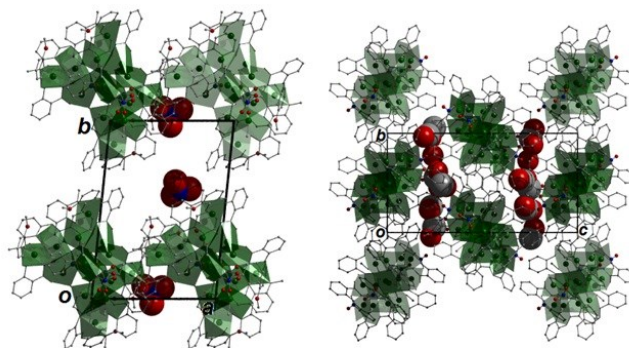
Figure 7 (Left) Polyhedral packing diagram of 2 as viewed along the c unit cell axis. Only the non-coordinating NO 3 - anions are shown in the space-fill mode. (Right) Polyhedral representation of the packing in 4 as viewed along the a axis of the unit cell. MeOH solvents of crystallisation are represented using the space-fill mode.
