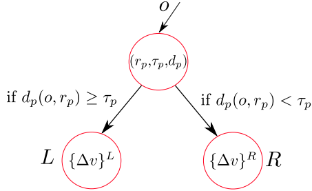
Figure 5: Internal node at test time. The test compares distance d_p(o, r_p) between test window o and training sample r_p with the threshold \tau_p .
