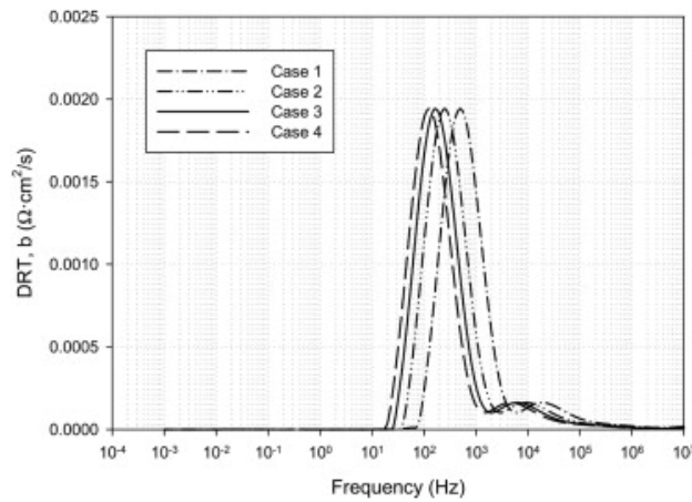
Figure A_II: DRT spectra for a finite length Warburg element with the values tabulated in Table A_II.
