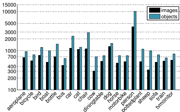
Fig. 2: Summary of the main VOC2012 dataset. Training and validation images only. Histogram by class of the number of objects and images containing at least one object of the corresponding class. Note the log scale on the vertical axis. Best viewed in colour.
