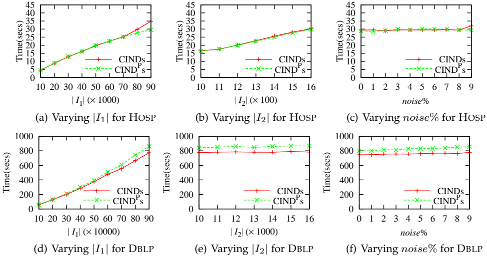
(a) Varying |I_1| for HOSP (b) Varying |I_2| for HOSP (c) Varying noise\% for HOSP (d) Varying |I_1| for DBLP (e) Varying |I_2| for DBLP (f) Varying noise\% for DBLP
