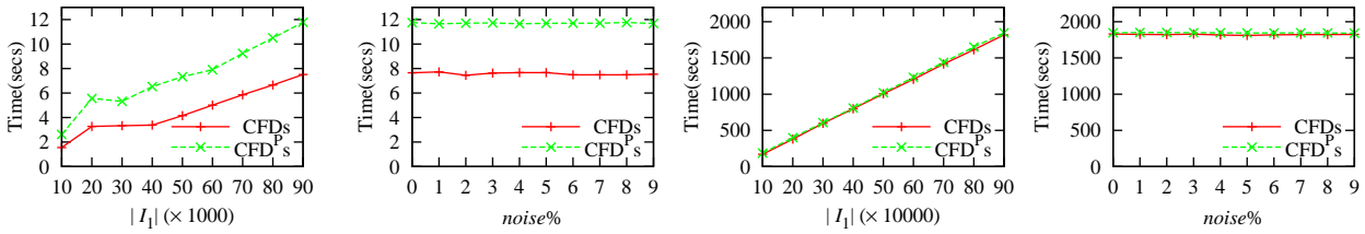
(a) Varying |I_1| for HOSP (b) Varying noise\% for HOSP (c) Varying |I_1| for DBLP (d) Varying noise\% for DBLP
