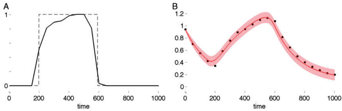
Fig. 4. Modelling results on the toy data, for one target gene. (A) Predicted promoter state \mu_i(t) (solid line) versus true state (dashed line). (B) Posterior mean of gene expression x_i(t) , with confidence intervals. Points show observed expression \bar{x}_i
