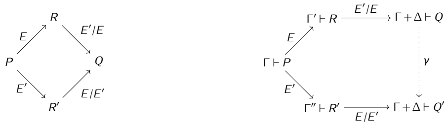
Figure 5: Cofinality in the style of CCS (left); with explicit braiding (right)
