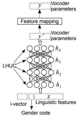
Figure 1: Three ways to do speaker adaptation for DNN-based speech synthesis. LHUC=Learning Hidden Unit Contributions.
