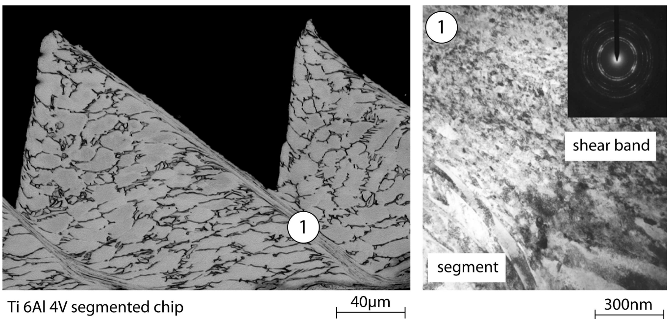
FIG. 3: Imaging the localized shear-band. Left: Optical microscopy image of a Ti6Al4V segmented chip produced in orthogonal high-speed cutting at v_c = 10 m/s; a_p = 0.1 mm. The average \alpha grain size in the segments is 20 \mu\text{m} . Right: Detail from position 1 showing that the shear band consists of equiaxed, nano-crystalline \alpha -grains. The average grain size is about 10 nm. The shear band can be clearly distinguished from the segment. The SAD (inset) shows that metastable \beta -phase is not present. Supplemental Fig.6 shows the same behaviour in a \beta -Ti alloy
