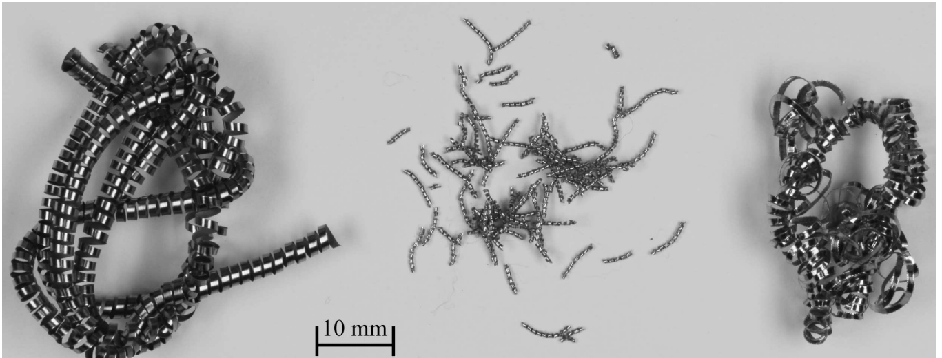
FIG. 2: Chips from conventional turning experiments. From left to right, chips of standard Ti6Al4V, and with addition of 0.9wt% La and 0.9wt% Er. Chip analyses show that only the La-containing material exhibits sufficient shear-band softening to fracture the chip. The effect of La on larger scale chip morphology is self-evident.
