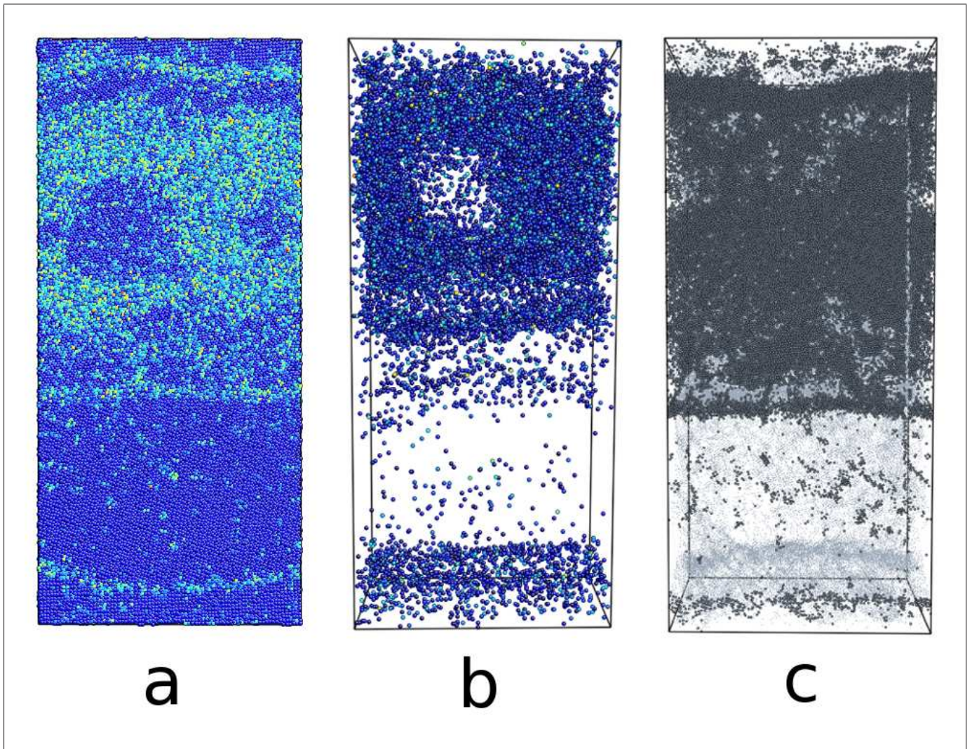
FIG. 1: Dynamical Phase Transition Snapshots from molecular dynamics simulation at 1500K and 55% strain at a rate of 2.5 \times 10^8 showing shear localization and amorphization imaged by Atomeye software[33]. (a) Slice through the system identifies atoms by centrosymmetry parameter, blue indicates atoms in close to bcc configurations. (b) 3D projection of only those atoms identified as non-crystalline. The separation between amorphous localized shear-band and crystalline region is clear, with the “hole” indicating a nanocrystal “floating” in the amorphous zone (c) 3D projection showing only those atoms with fewer than 10 of their original 14 neighbours, showing that shear and diffusion has been largely confined to the amorphous layer.
