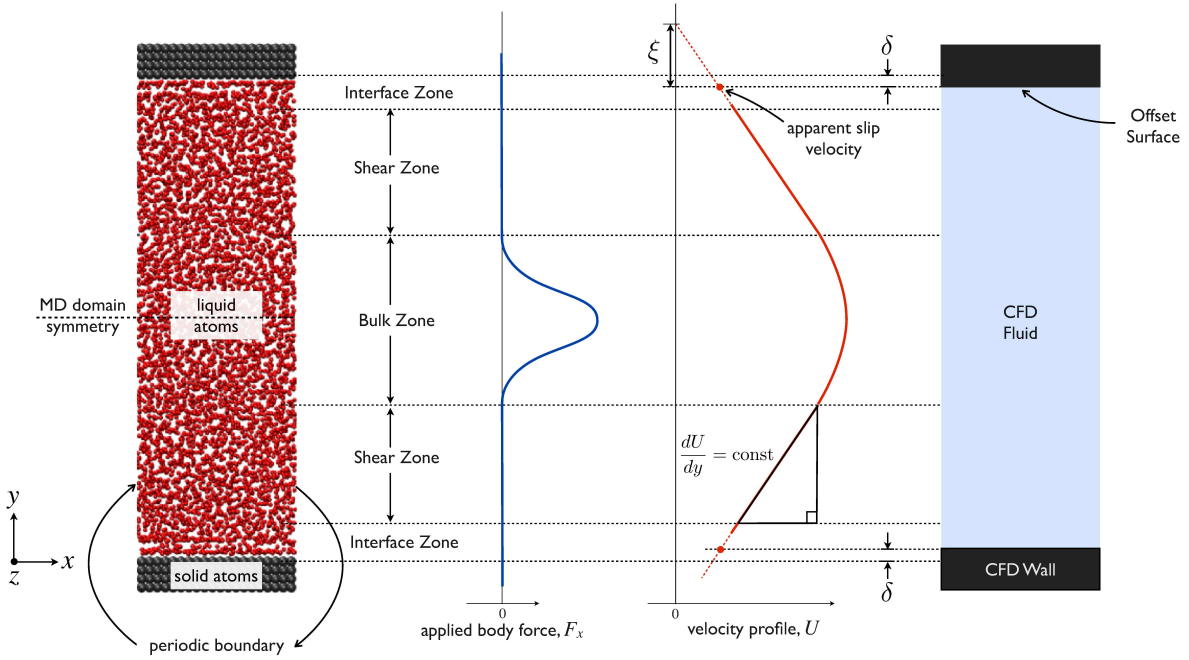
Fig. 1 Schematic of Molecular Dynamics pre-simulation for extracting fluid dynamic properties that are essential inputs to an enhanced CFD solver for nano-scale flows.
