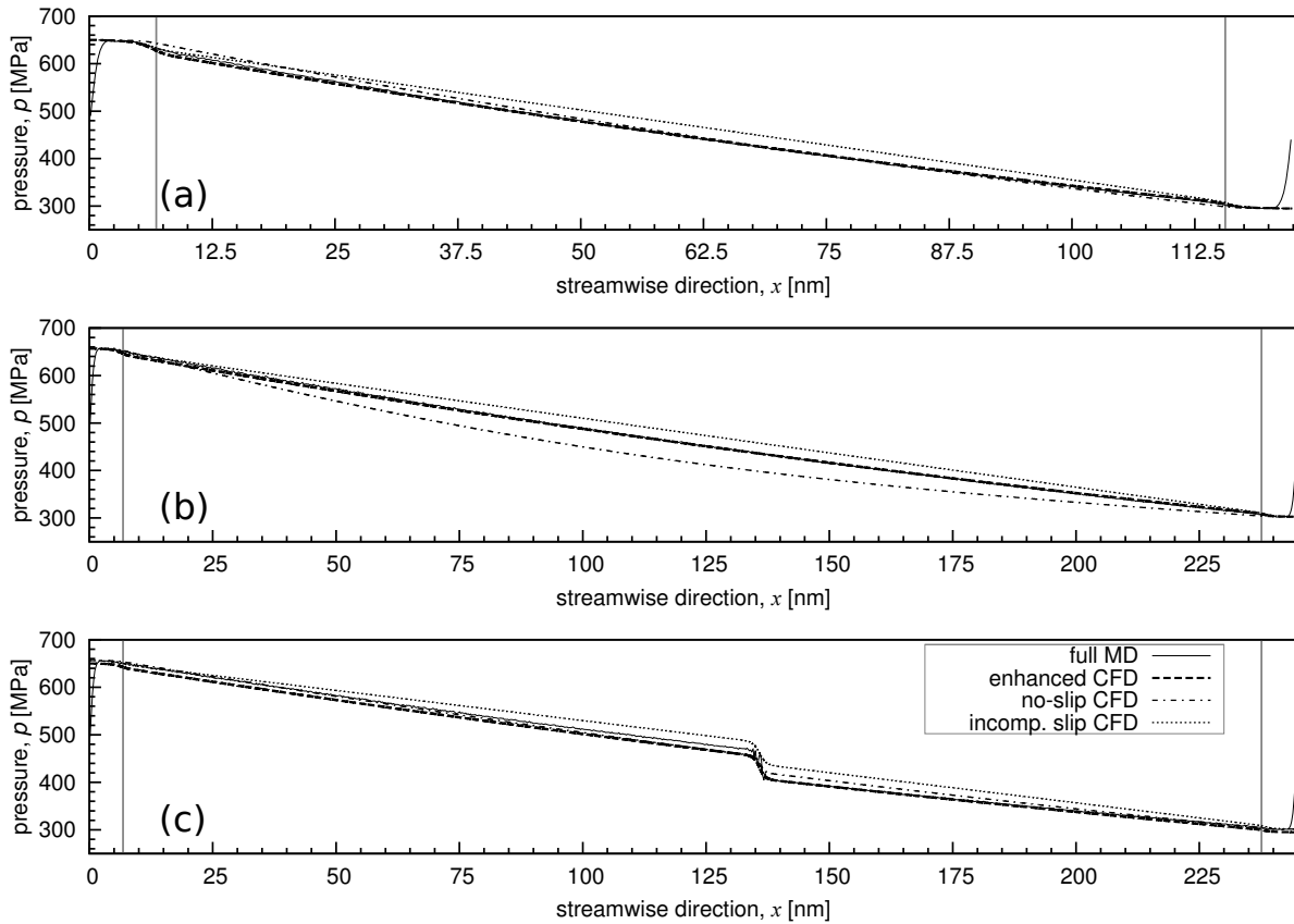
Fig. 7 Pressure along the centerline of (a) Case 1 (short channel), (b) Case 2 (long channel), and (c) Case 3 (defect channel). The vertical lines at x = 6.8 nm and x = 115.6 nm (for Case 1) and at x = 6.8 nm and x = 238 nm (for Cases 2 and 3), indicate the inlet and outlet positions, respectively. Full MD (—), enhanced CFD (---), no-slip CFD (-.-) and incomp. slip CFD (···).
