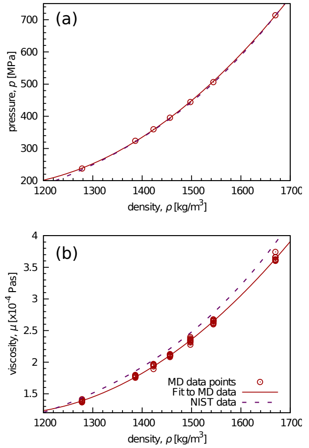
Fig. 2 Data for the Lennard-Jones fluid properties: (a) pressure variation with density, and (b) viscosity variation with density. MD data points from pre-simulation (circles), fitted polynomial (solid lines) and NIST data (Linstrom and Mallard, 2001) (dashed lines).
