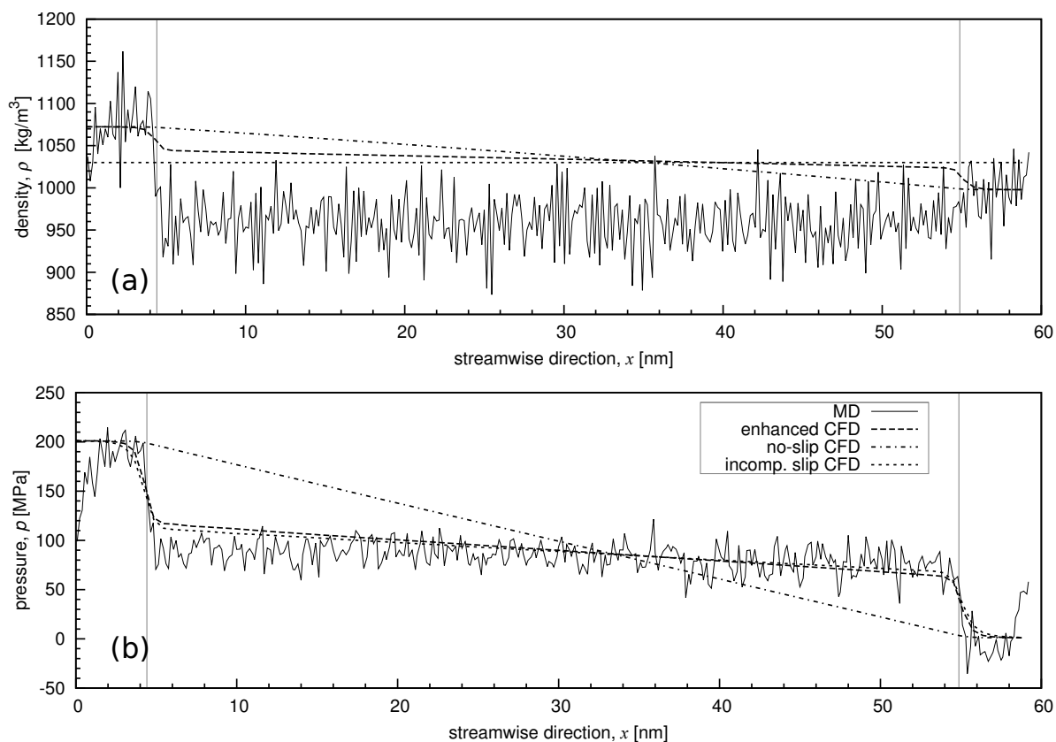
Fig. 11 Water density and pressure along the centerline of the CNT. The noise in the MD data is due to the relatively small number of molecules being sampled in the absence of a well defined ‘bulk-flow’ region. The vertical lines at x = 4.4 nm and x = 55.8 nm represent the inlet and outlet, respectively. Full MD (—), enhanced CFD (---), no-slip CFD (-·-) and incomp. slip CFD (···).
