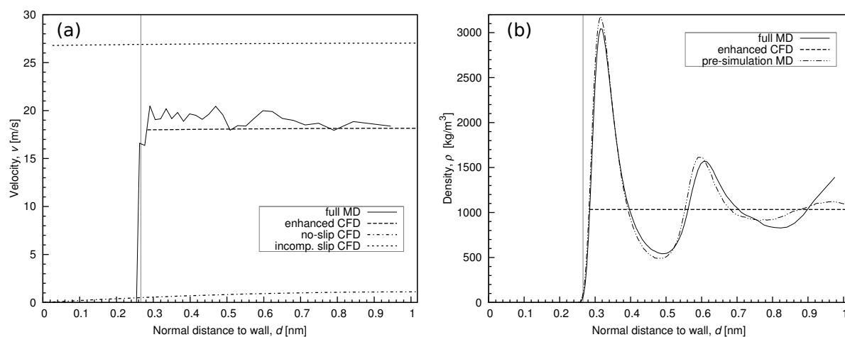
Fig. 12 (a) Streamwise velocity cross-sectional profile in the longitudinal center of the CNT, and (b) the radial water density profile within the CNT. The vertical lines at x = 0.266 nm indicate the position of the CFD surface; the CNT surface atom centres are at x = 0 .
