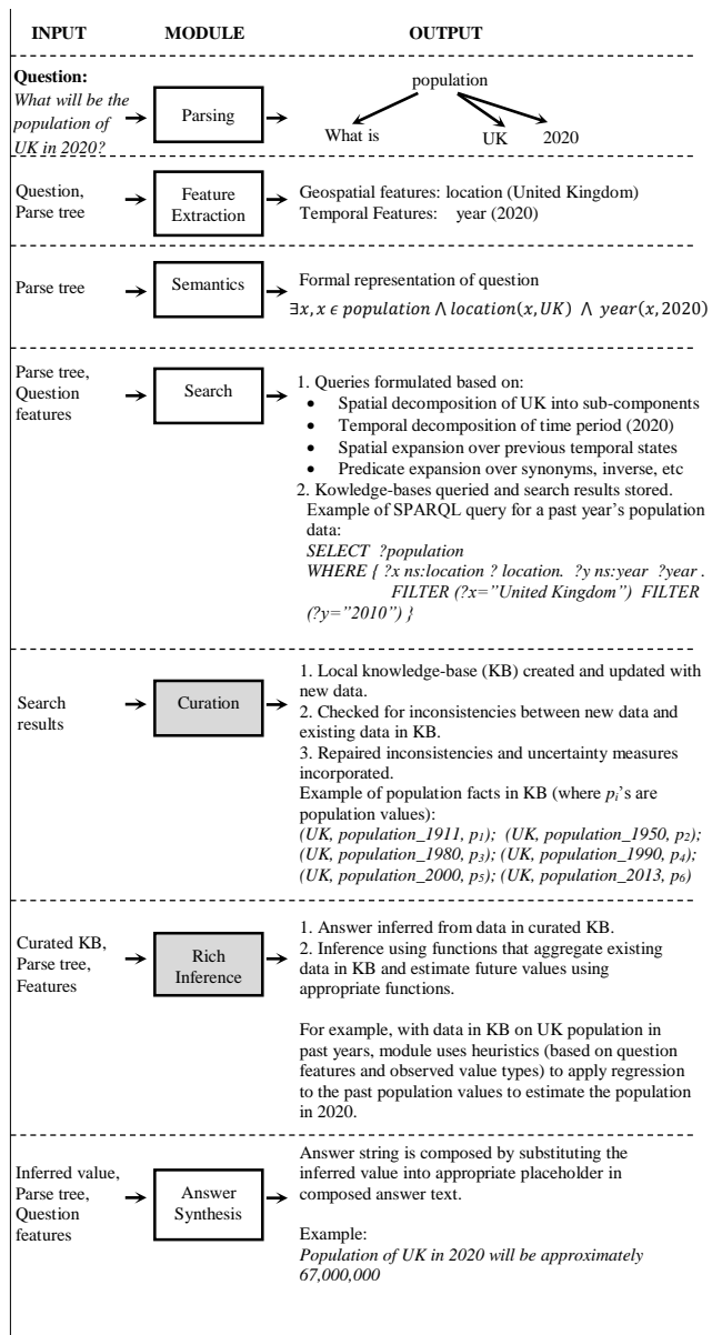
Fig. 5. Module inputs and outputs. Shaded modules represent the primary contributions of this project.
