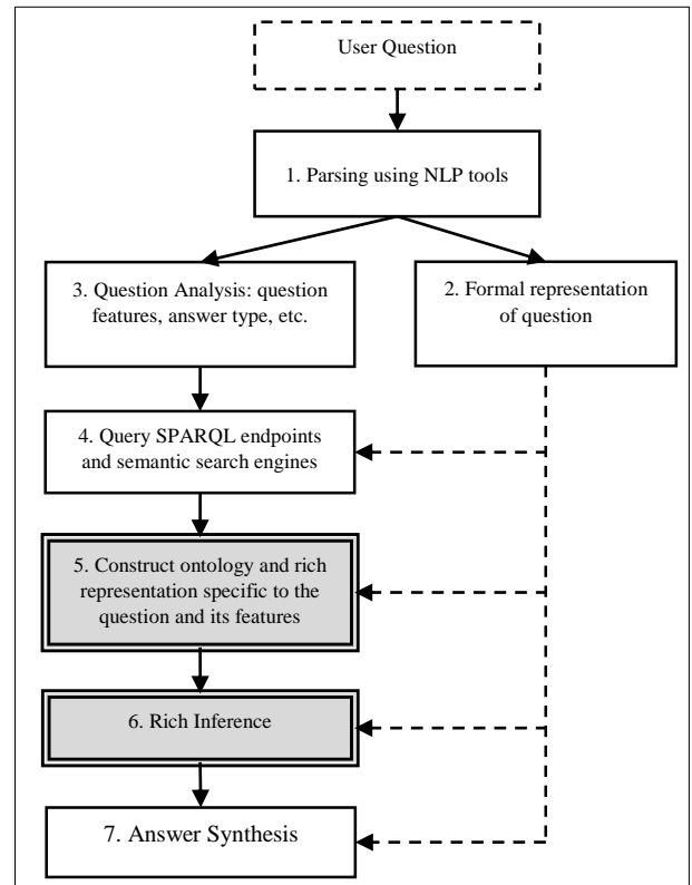
Fig. 4. QA pipeline. Shaded modules represent the primary contributions of this project
