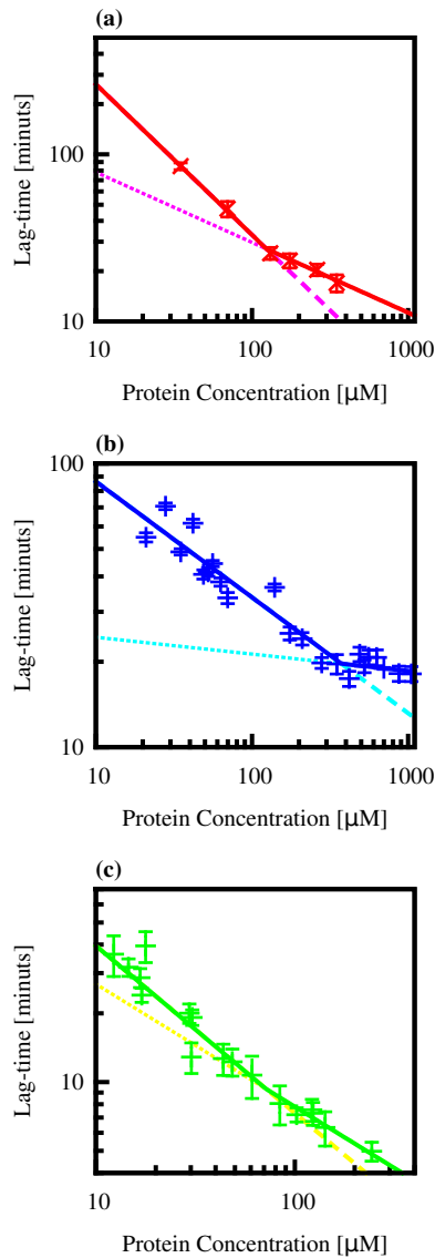
Figure 1: Lag time as a function of protein concentration for (a) bovine insulin, (b) lysozyme, and (c) \beta_2 microglobulin, in all cases averaged over replicate experiments. The data in (c) was kindly provided by Xue et al. (9). The error bars indicate the standard deviation among replicate experiments at a given concentration, and the lines indicate the best fit of the power law \tau_{\text{lag}} \propto m_{\text{tot}}^{-\gamma} to data for a specified range of protein concentrations. (a) shows two data sets for bovine insulin: the black data fitted by the single power law over all protein concentrations (resulting in \gamma = 0.36 ) indicates experiments in the absence of NaCl, while those in red fitted by two power laws indicate self-assembly in the presence of 0.49 M NaCl; each point corresponds to the mean and standard deviation of 140–200 kinetic traces at each of 6 protein concentrations (see Methods). Fitting the data for bovine insulin in the presence of NaCl in the range m_{\text{tot}} \leq 160 \mu\text{M} results in \gamma = 0.90(2) (dashed line); while fitting the data in the range m_{\text{tot}} \geq 160 \mu\text{M} results in \gamma = 0.42(10) (dotted line). (b) shows data for lysozyme (for conditions see Methods), where each point corresponds to the mean and standard deviation of 12–60 kinetic traces at each of 25 protein concentrations (see Methods). Fitting this data for in the range m_{\text{tot}} \leq 300 \mu\text{M} results in \gamma = 0.41(6) (dashed line); while fitting the data in the range m_{\text{tot}} \geq 300 \mu\text{M} results in \gamma = 0.06(5) (dotted line). (c) shows data for \beta_2 microglobulin, where each point corresponds to the mean and standard deviation of 235 kinetic traces at 20 different protein concentrations (for conditions see Methods and Xue et al. (9)). Fitting the data in the range m_{\text{tot}} \leq 40 \mu\text{M} gives \gamma = 0.77(14) (dashed line), while fitting the data in the range m_{\text{tot}} \geq 40 \mu\text{M} gives \gamma = 0.54(5) (dotted line).
