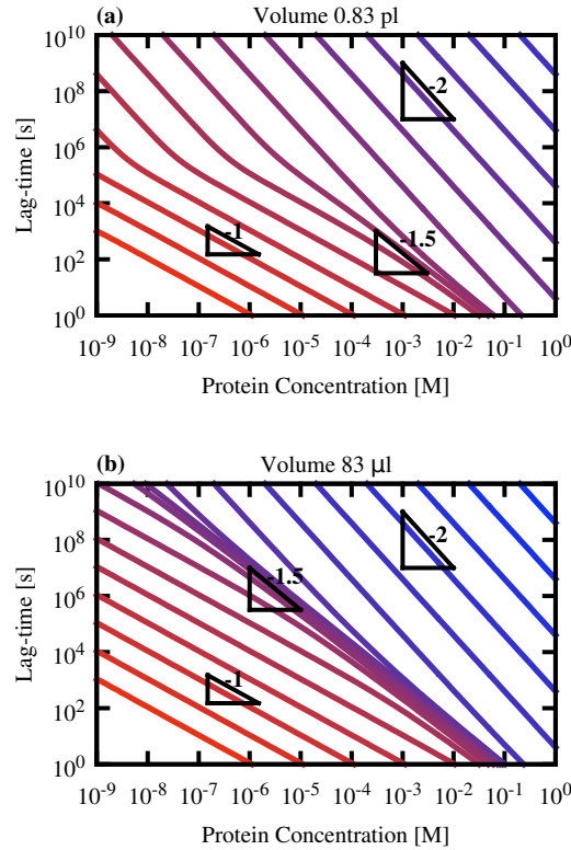
Figure 4: Kinks are also predicted in lag-time versus concentration curves for a model where the autocatalysis mechanism is provided by secondary nucleation. Lag-time versus concentration curves predicted by Eq. 9 are shown for a series of values of the primary nucleation rate k_n (increasing top right to bottom left) from 10^{-30} \text{ M}^{-1} \text{ s}^{-1} (blue) to 10^6 \text{ M}^{-1} \text{ s}^{-1} (red), increasing by factors of 100. The two panels show results for different system volume V : (a) corresponds to V = 0.83 \text{ pl} (approximately the size of a human cell) while (b) corresponds to the much larger volume V = 83 \text{ } \mu\text{l} (a typical volume used in in vitro protein aggregation experiments). The other parameters are k_+ = 5 \times 10^4 \text{ M}^{-1} \text{ s}^{-1} , k_s = 24 \text{ M}^{-1} \text{ s}^{-1} , n_c = 2 and n_s = 2 .
