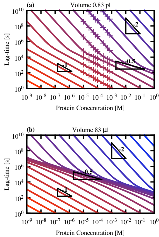
Figure 3: Transitions between different scaling regimes appear as kinks in lag-time versus concentration curves. Lag-time versus concentration curves predicted by Eq. 9 are plotted for a range of primary nucleation rates k_n . k_n increases top right to bottom left and is colour-coded from k_n = 10^{-30} \text{ M}^{-1} \text{ s}^{-1} (blue) to k_n = 10^{10} \text{ M}^{-1} \text{ s}^{-1} (red), being increased by factors of 100. The two panels show results for different system volume V : (a) corresponds to V = 0.83 \text{ pl} (approximately the size of a human cell) while (b) corresponds to the much larger volume V = 83 \text{ µl} (a typical volume used in in vitro protein aggregation experiments). In (a), the crosses correspond to the simulation data given of Fig. 2a. In all cases, k_+ = 5 \times 10^4 \text{ M}^{-1} \text{ s}^{-1} , k_f = 3 \times 10^{-8} \text{ s}^{-1} and n_c = 2 .
