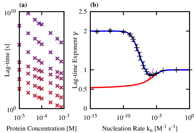
Figure 2: Lag-time scaling with protein concentration for the fragmentation model depends on the primary nucleation rate constant. (a) Lag-time versus concentration curves obtained from stochastic simulations, for several values of the nucleation rate constant k_n : k_n increases top to bottom in factors of 100, from 10^{-12} M -1 s -1 (purple) to 1 M -1 s -1 (red). (b) Lag-time scaling exponent \gamma as a function of primary nucleation rate constant k_n . Black symbols: simulation results obtained by fitting the data shown in (a) to \log(\tau_{\text{lag}}) = \log(A) - \gamma \log(m_{\text{tot}}) . The error bars are dominated by the confidence in the fit, rather than the error in the lag-time measurements. Red line: \gamma(k_n) extracted from the full prediction of the fragmentation model, Eq. 7. Magenta line: \gamma(k_n) extracted from the approximate prediction of the fragmentation model, Eq. 8. Blue line: \gamma(k_n) extracted from the lag-time expression Eq. 9 — i.e., the full fragmentation model solution augmented by an extra term to describe the first primary nucleation event. For all the data shown, the protein concentration range was 1 \times 10^{-5} \leq m_{\text{tot}} \leq 7.5 \times 10^{-4} M and the parameters were n_c = 2 , k_+ = 5 \times 10^4 M -1 s -1 , k_f = 3 \times 10^{-8} s -1 and the volume V = 0.83 pl.
