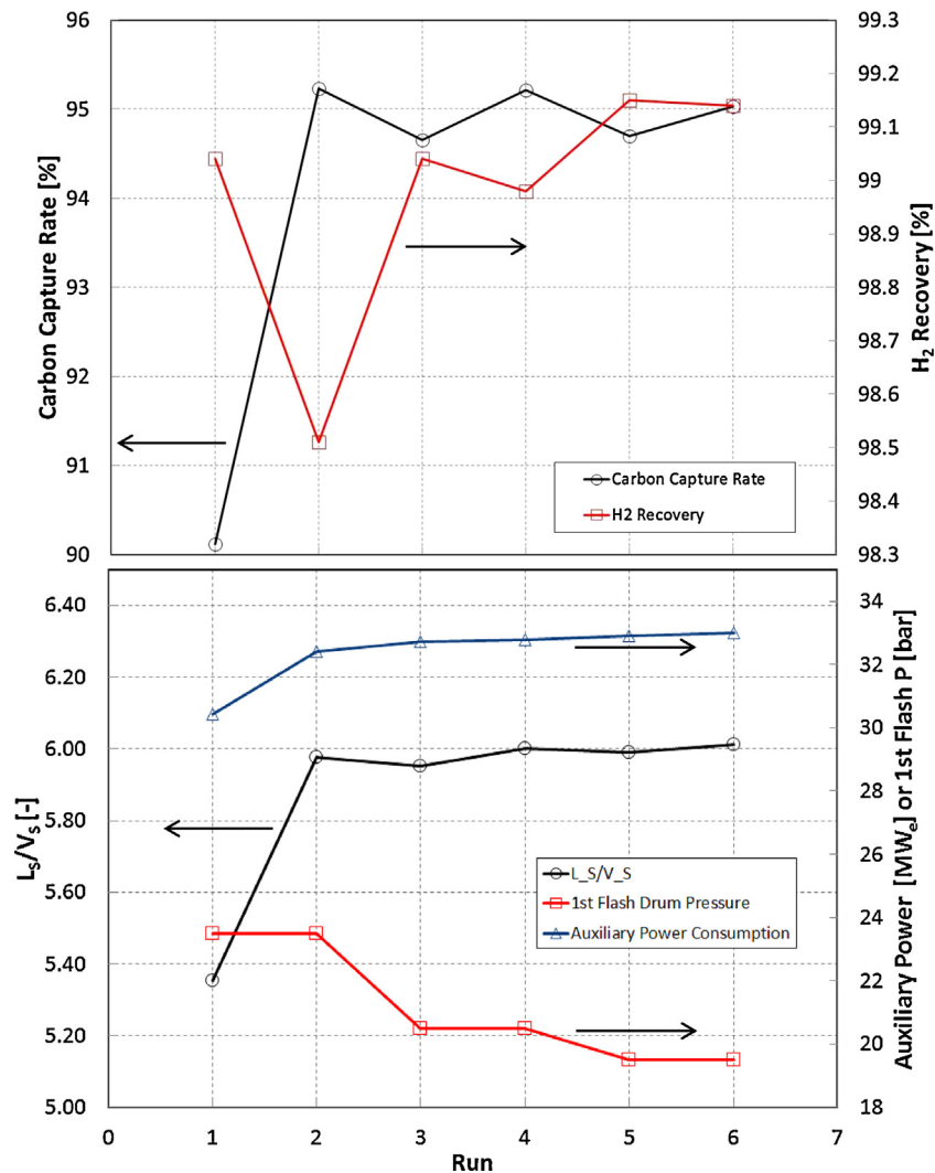
Fig. 6. Change of performance and operating conditions over the simulation runs of an integrated dual-stage Selexol process for increasing the carbon capture rate from 90% to 95%.
