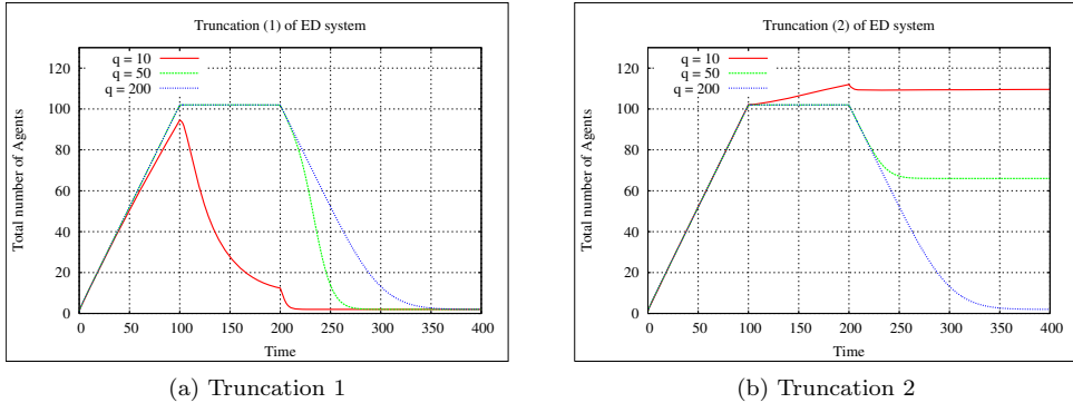
Figure 9. Numerical integration of truncations 1 and 2 up to F_{10} , F_{50} , and F_{200} . Rates and initial states are as in the stochastic case. The quality of the approximation for truncation 2 degrades clearly for F_{50} compared to truncation 1.
