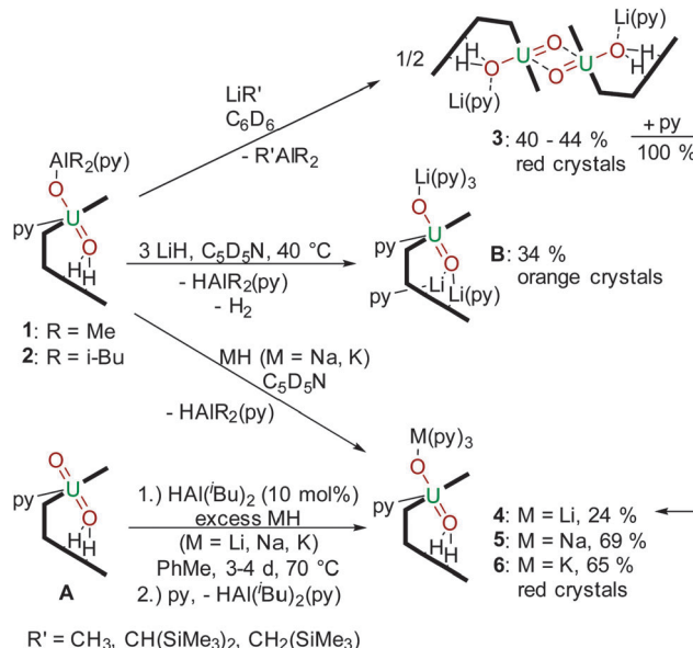
Scheme 2 Transmetalation reactions of 1 and 2 with R'Li, LiH, NaH and KH, and the HA( i -Bu) 2 -catalysed reduction of [U VI O 2 (H 2 L)] by MH.
