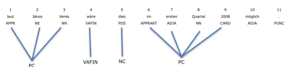
Figure 7: Chunked sentence
