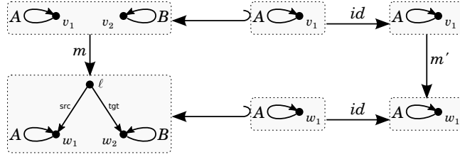
Fig. 2: An example pushout in \mathbf{bG}_* . Horizontal spans represent partial maps. Vertical maps m, m' are total and send v_i to w_i for i \in \{1, 2\} .
