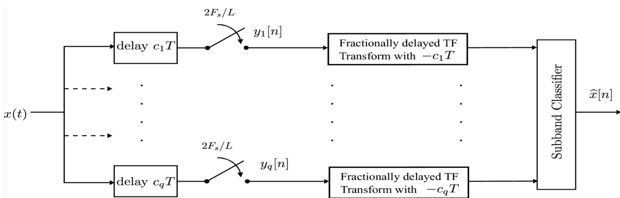
Figure 1: The proposed low-complexity sub-Nyquist sampling system.
