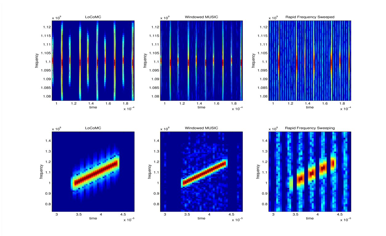
Figure 3: ESM signal reconstruction using proposed method (left) the subspace method (middle) and rapid frequency sweeping (right).
