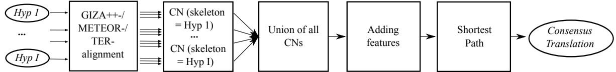
Figure 1: Confusion network decoding structure.
