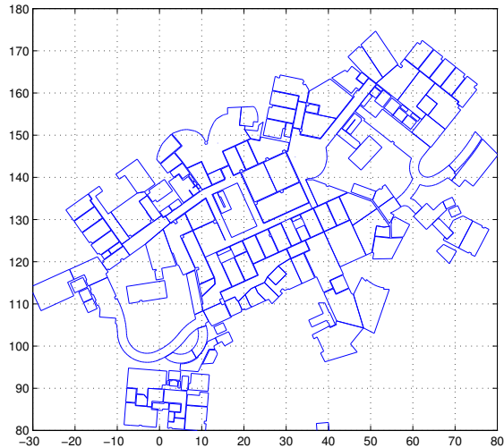
Fig. 3. Floorplan of the 3rd floor of the Stata Center, with units in meters.
