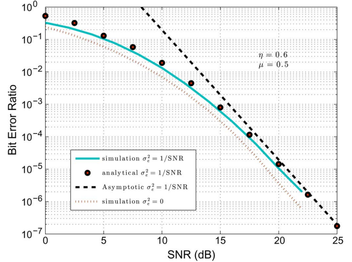
Fig. 11. Average BER performance of the SSK 4 \times 4 MIMO system versus SNR for \eta = 0.6 and \mu = 0.5 .
