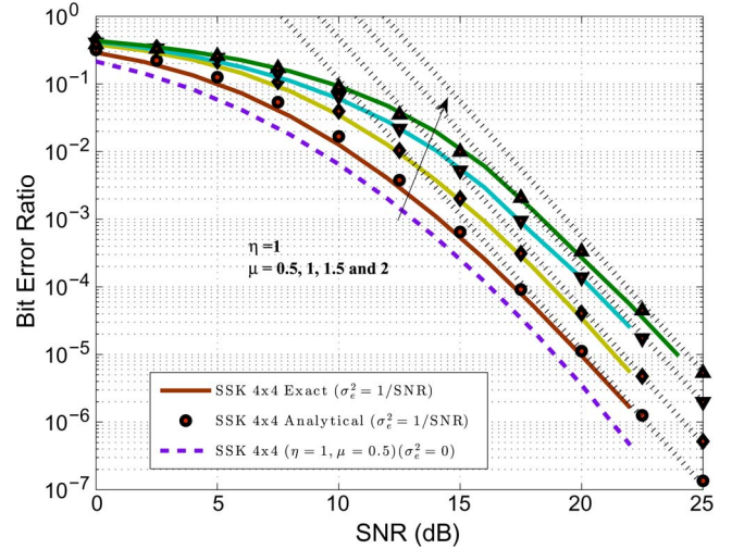
Fig. 10. Average BER performance of the 4 \times 4 MIMO SSK system versus SNR for different values of \mu and \eta = 1 .
