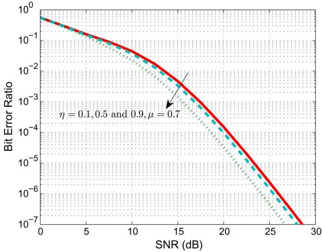
Fig. 9. Impact of changing the \eta parameter on the performance of the SM system for a fixed value of \mu = 0.7 .
