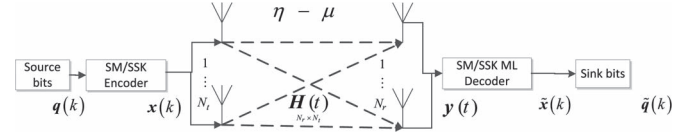
Fig. 1. SM/SSK system model over \eta-\mu MIMO fading channel.
