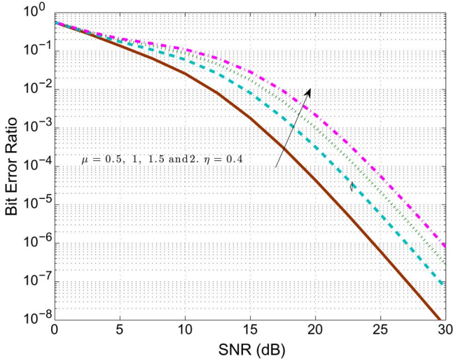
Fig. 8. Impact of changing the \mu parameter on the performance of the SM system for a fixed value of \eta = 0.4 .
