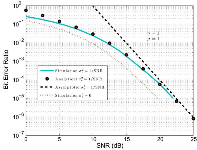
Fig. 5. Average BER performance of an SM system versus SNR for \mu = 1 and \eta = 1 .
