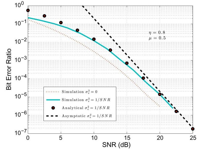
Fig. 7. Average BER performance of an SM system versus SNR for \mu = 0.5 and \eta = 0.8 .
