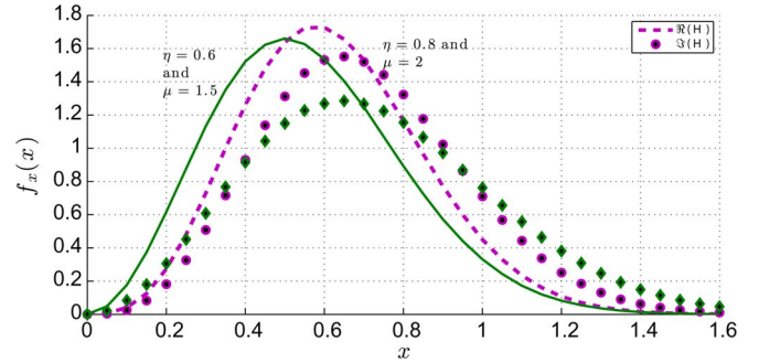
Fig. 3. Numerical estimation of the PDFs of the real and imaginary parts of the complex \eta - \mu channel.
