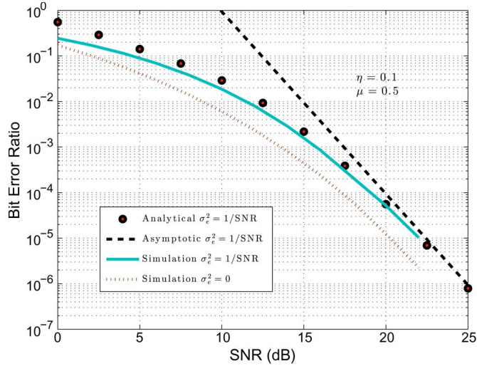
Fig. 4. Average BER performance of the SM system versus SNR for \mu = 0.5 and \eta = 0.1 .
