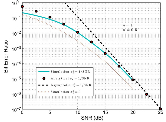
Fig. 6. Average BER performance of an SM system versus SNR for \mu = 0.5 and \eta = 1 .
