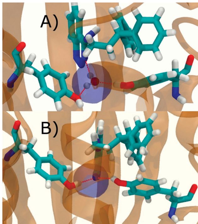
Fig. 6 Representation of GCT monitored regions in scytalone dehydratase. (A) In complex with 1 (B) in complex with 2 . Regions s_{AP} and s_{BP} are depicted by the transparent blue spheres for r_c = \text{full} and X_{\text{medoid}} = 4 \text{ \AA} . The regions obtained with r_c = \text{bb} and X_{\text{medoid}} = 4 \text{ \AA} conditions are not shown because they are similar. Relevant hydrogen-bonding interactions between protein residues, water molecules and ligands are depicted by red-dotted lines.
