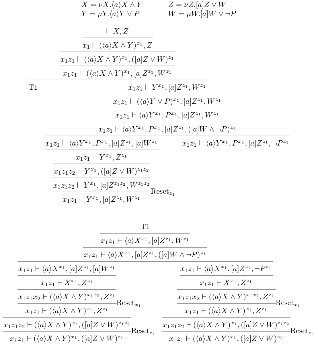
Figure 8: A proof tree
