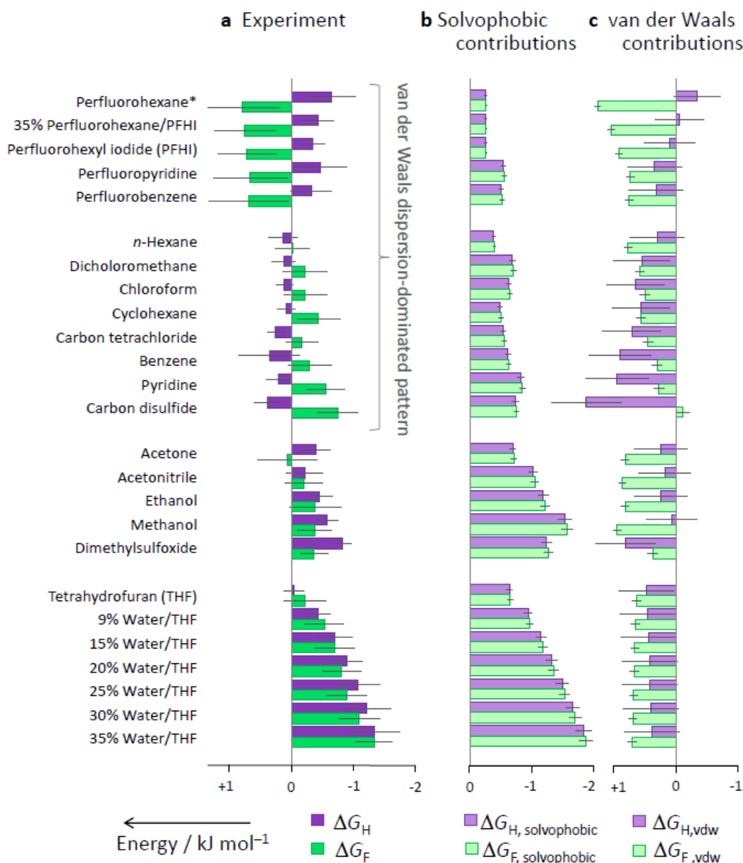
Figure 2. a) Experimental cohesive interaction energies measured between alkyl chains, \Delta G_H (purple) and perfluoroalkyl chains, \Delta G_F (green) using molecular balances ( \pm )-1H to ( \pm )-4H and ( \pm )-1F to ( \pm )-4F and Equations 1 and 2, respectively. All solvent mixtures are reported in % v/v. b) Dissected solvophobic ( \Delta G_{\text{solvophobic}} ) and c) van der Waals ( \Delta G_{\text{vdw}} ) free energy contributions to alkyl-alkyl (light purple) and
